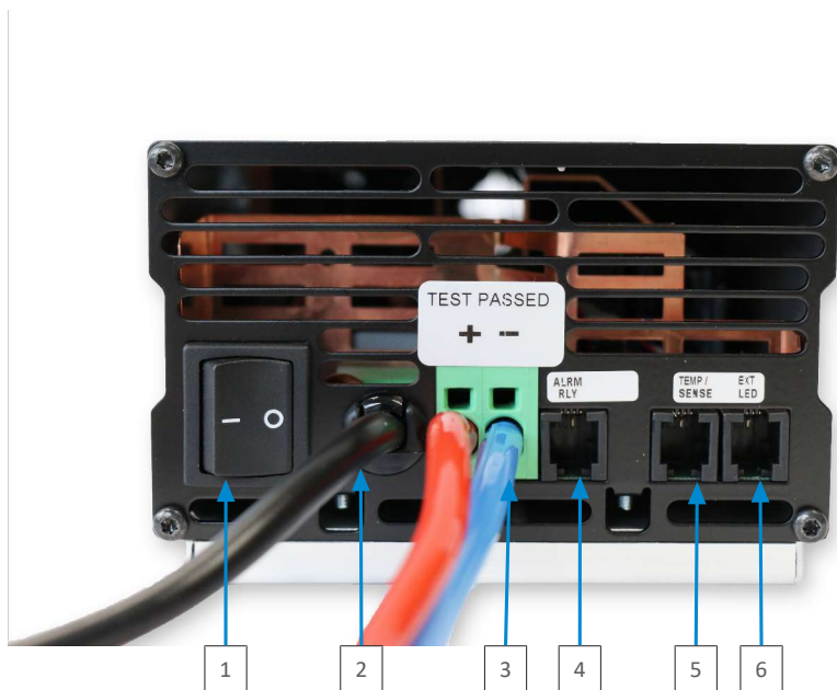
Fig. 2: ABC charger connection side
